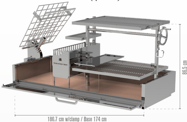
Front view (open door)
